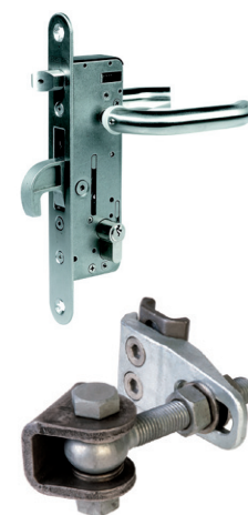
boven: Locinox Hybrid Lock onder: detail 180°scharnier
